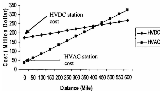
Fig. 1. HVDC and HVAC Transmission systems cost
