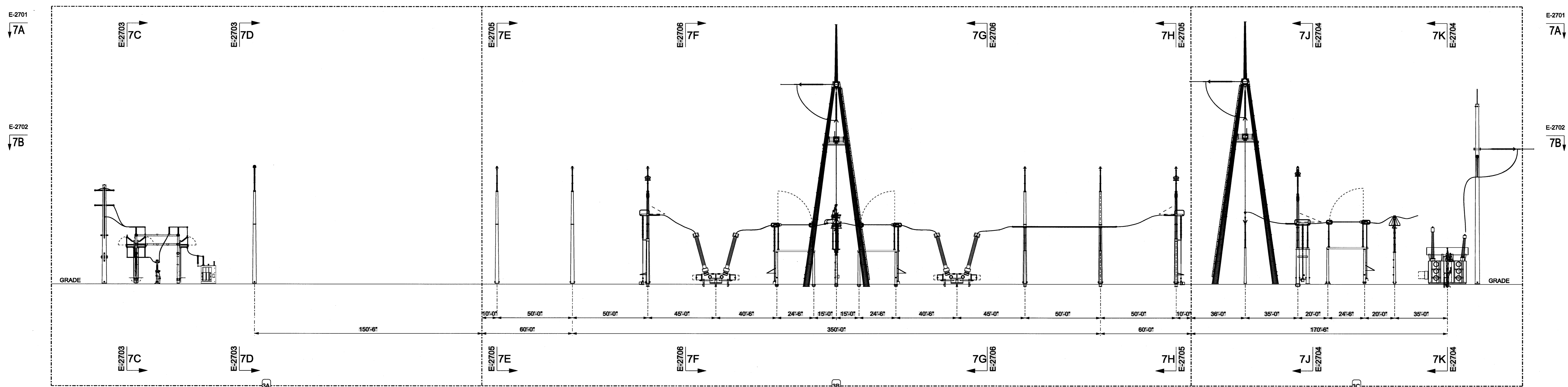
SECTION "7N3-7N3"
